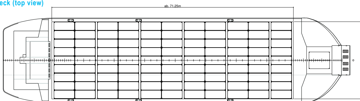
Weather deck (top view)
